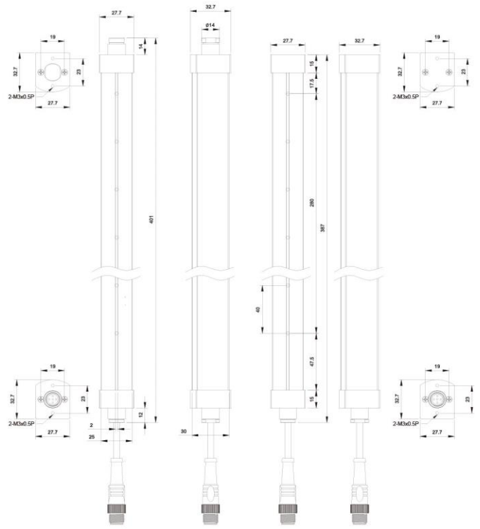
XH8-1(5)M□-U6-40
