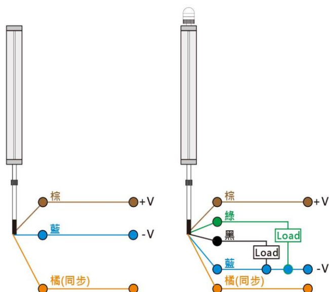
PNP NO&NC Type
