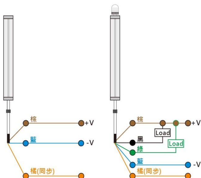
NPN NO&NC Type
