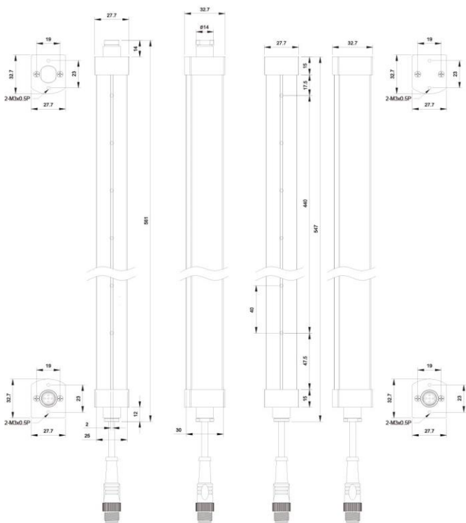
XH12-1(5)M□-U6-40
