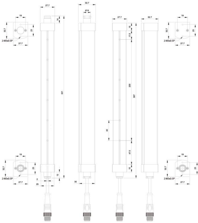
XH6-1(5)M□-U6-40
