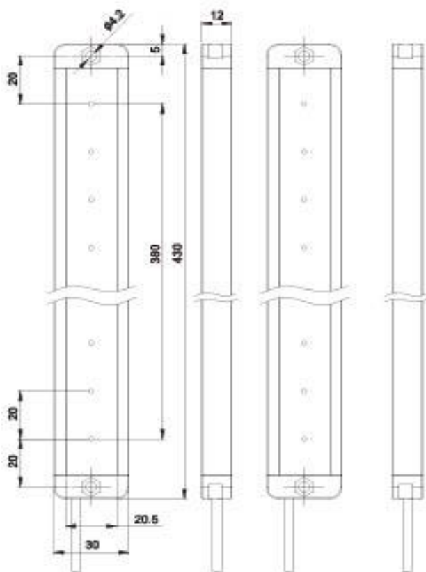
XH20-2M□-U5
