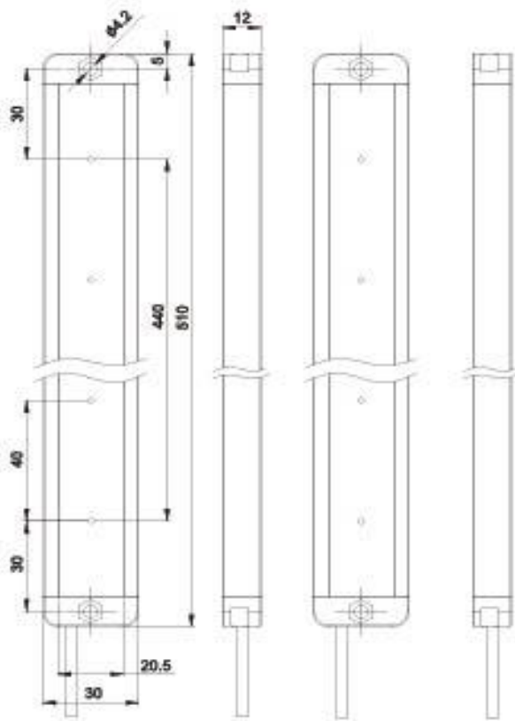
XH12-2M□-U5-40
