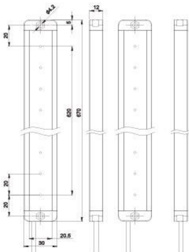
XH32-2M□-U5
