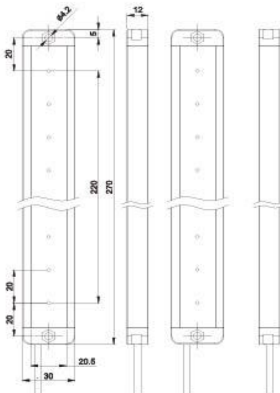
XH12-2M□-U5
