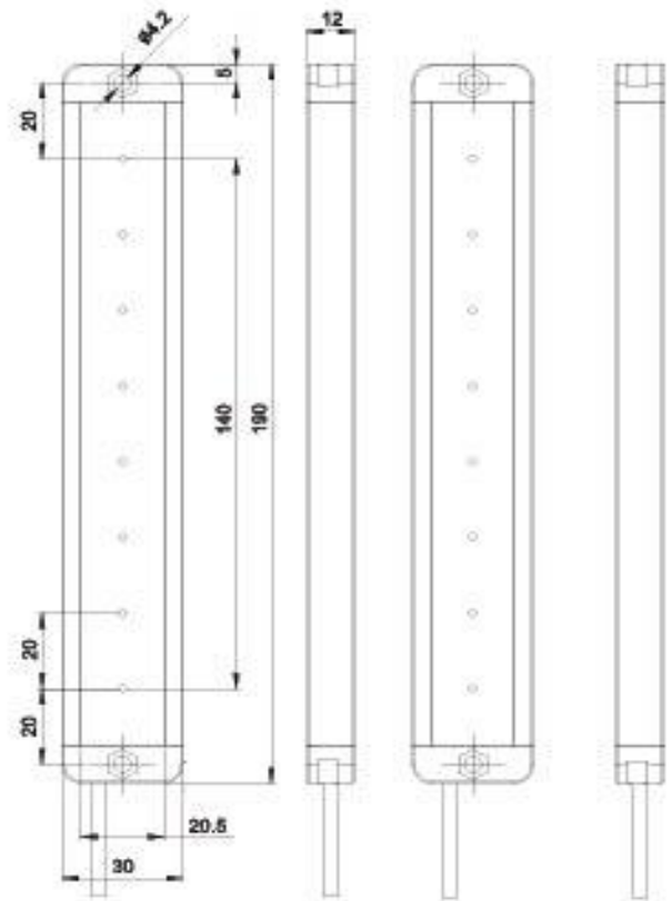
XH8-2M□-U5
