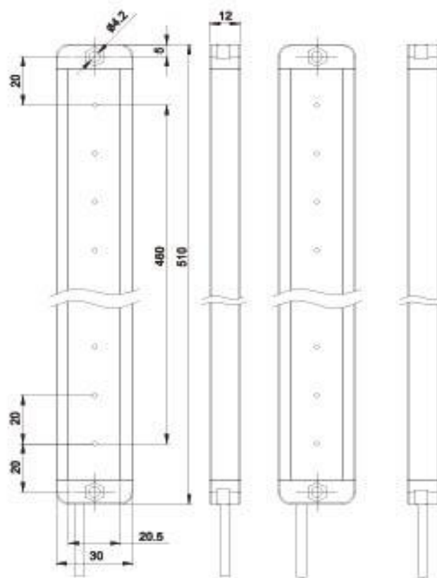
XH24-2M□-U5
